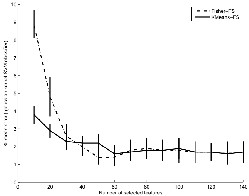
Fig. 3. Mean classification error rate (5 cross validation loops) obtained with a Gaussian kernel SVM after selection by two methods: Fisher-FS (supervised) and k -Means-FS (unsupervised), as a function of the number of selected features. The vertical lines represent one standard deviation apart from the mean error. Without selection the results are 1.7\% \pm 0.6\% . The best result with Fisher-FS is 1.4\% \pm 0.4\% (50 selected features) and with k -Means-FS 1.6\% \pm 0.5\% (60 selected features).
