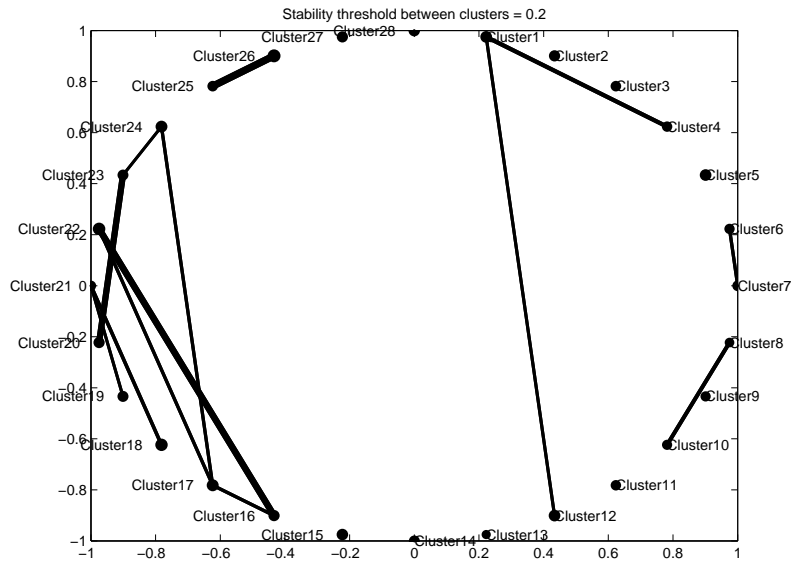
Fig. 4. Graph representing clusters and their connections. The thickness of each link is proportional to the value S_{inter} . Isolated clusters correspond to high S_{intra} values.
